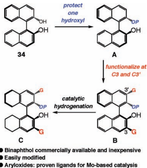
Scheme 6. Monoprotected Binaphthols: A Versatile Class of Chiral Monodentate Ligands
