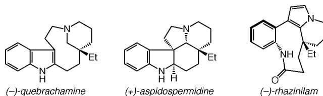
Scheme 1. Representative Members of the Aspidosperma Group of Alkaloid Natural Products
