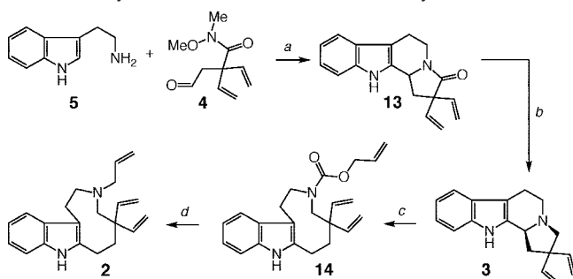
Scheme 4. Synthesis of the RCM Precursor, Tricyclic Triene 2 a
