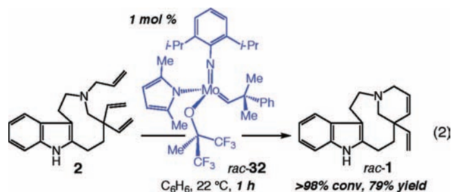
Scheme 6. Monoprotected Binaphthols: A Versatile Class of Chiral Monodentate Ligands
