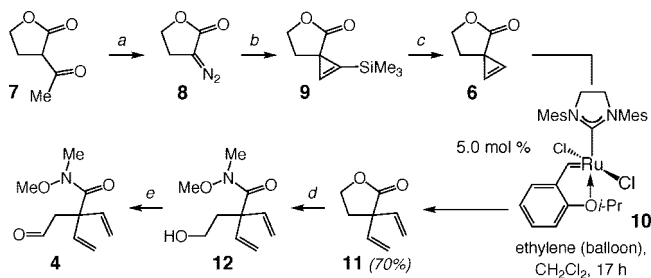
Scheme 3. Synthesis of Divinylamide Fragment 4 through Ru-Catalyzed ROCM a
