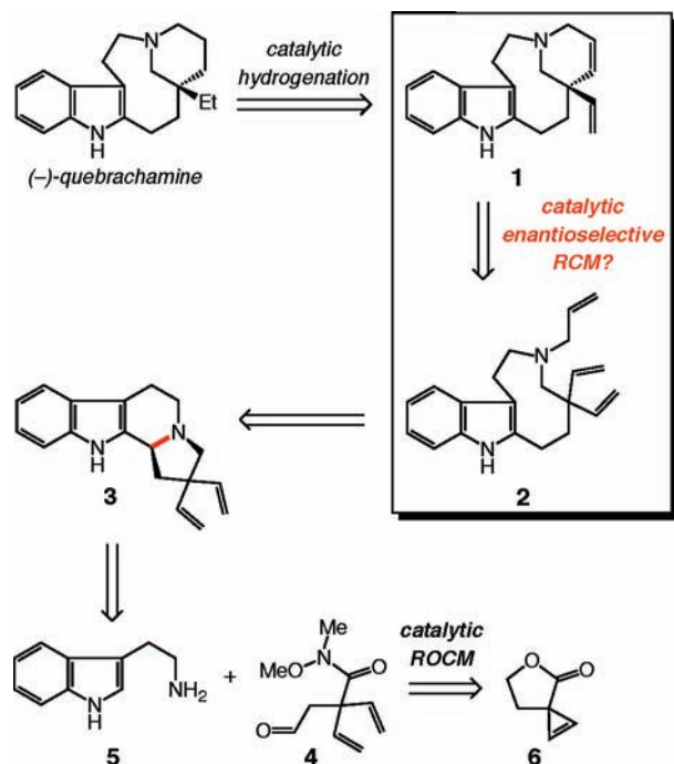
Scheme 2. Retrosynthesis Analysis for Enantioselective Preparation of Quebrachamine
